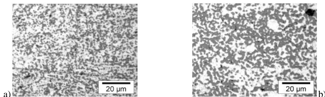
Figure 5: Pictures of the polished cross section (light microscopy) of nanostructured copper after SPS compaction at a) 700°C and b) 800°C.
