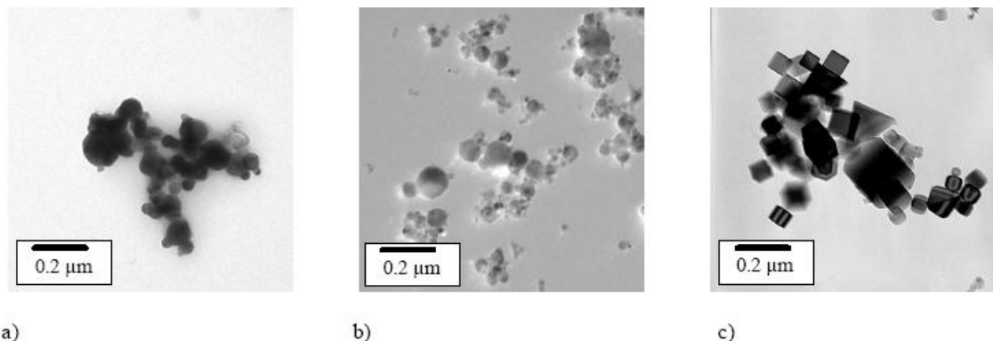
Figure 1: TEM micrographs of the investigated nanostructured powder before compaction: a) copper, b) titanium oxide, c) titanium carbonitride; field of view approximately 1μm.
