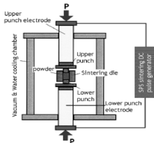
Figure 2: Schematic drawing of the applied SPS apparatus.
