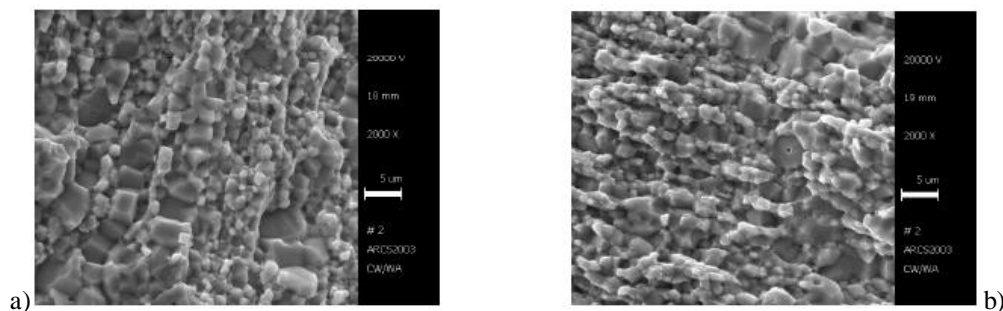
Figure 3: Scanning electron microscope (SEM) micrograph of nanostructured titanium carbonitride powder after compaction by means of SPS at a) 1600°C for 1 min (fracture surface) and b) 1800°C for 1 min (fracture surface).
