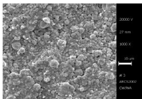
Figure 4: Scanning electron microscope (SEM) micrograph of nanostructured titanium carbonitride powder after compaction by means of GPS at 2100°C for 45 min (fracture surface).
