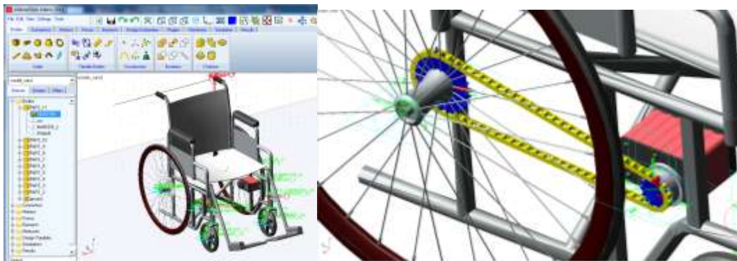
Fig. 4. Adams kinematic model and chain system in Adams Machinery.
