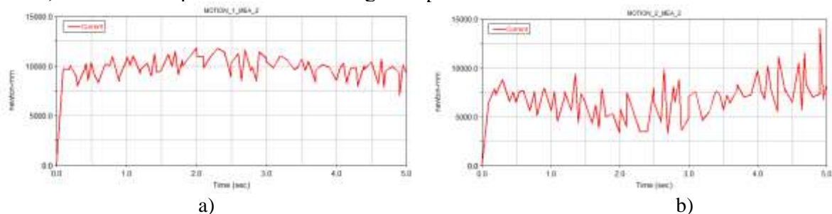
Fig. 6. Propulsion torque for wheelchair right wheel and left wheel.
