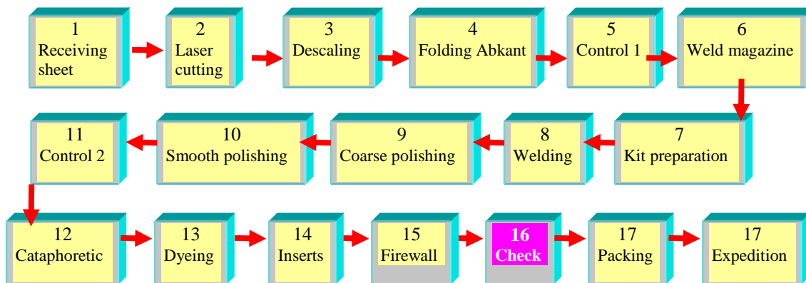
Figure 4. The technological production flow of study highlights control box now ameliorated
