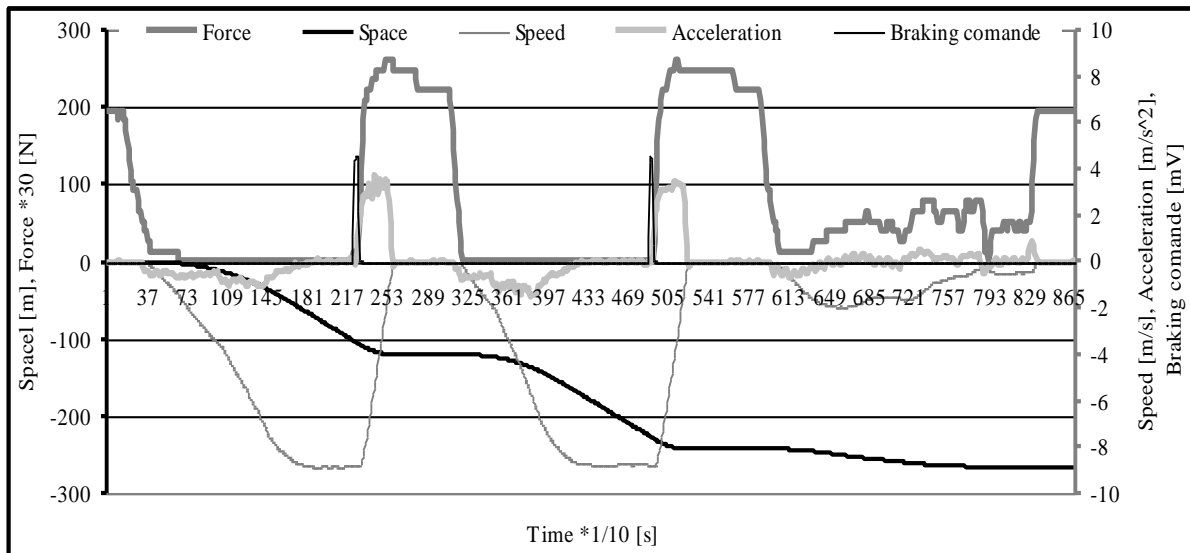
Fig.7. Right tie bar, left skip going down
