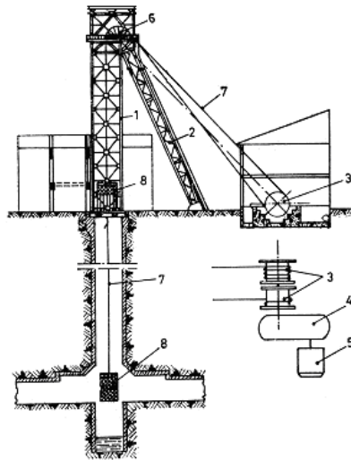
Fig.1. The principle draft of the extraction installation
