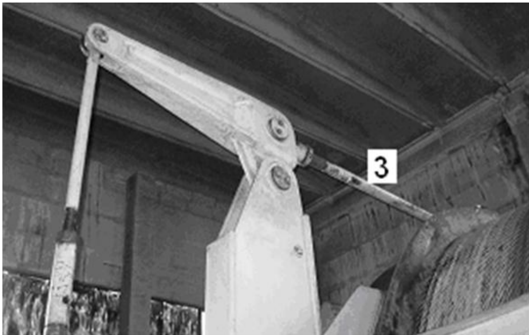
Fig.5. Tirant left wit tension metres marks
