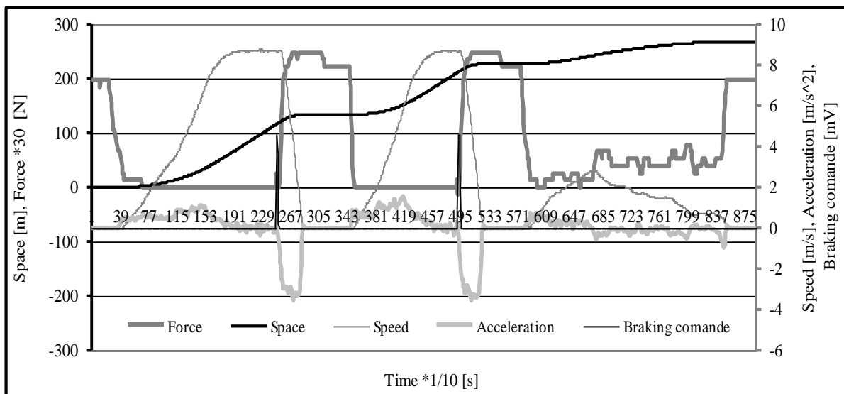
Fig.8. Right tie bar, left skip going up
