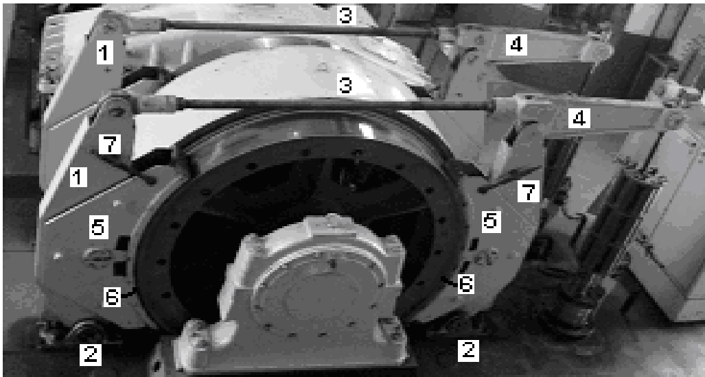
Fig.2. Braking–device extraction – machine
